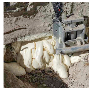
Underpinning bracket with integrated anchor and PolyLevel injection
